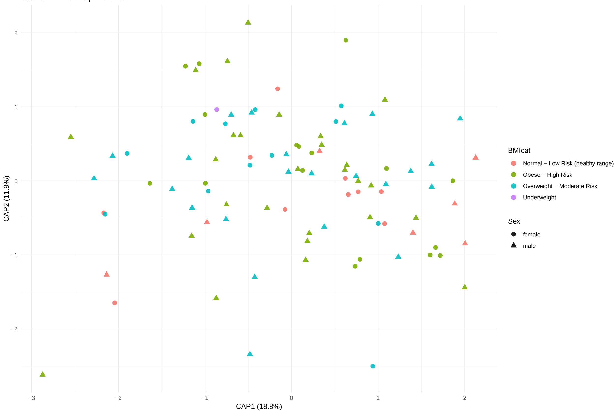
CAP Ordination by Multiple Variables adonis R^2 = 0.17 , p = 0.378
